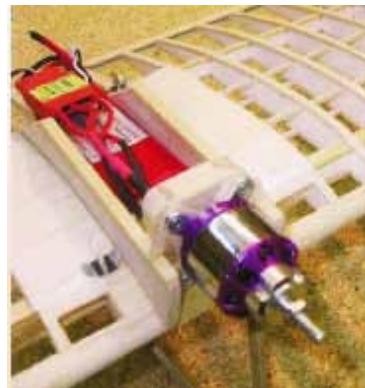
Typical of the four engine installations in the wing
